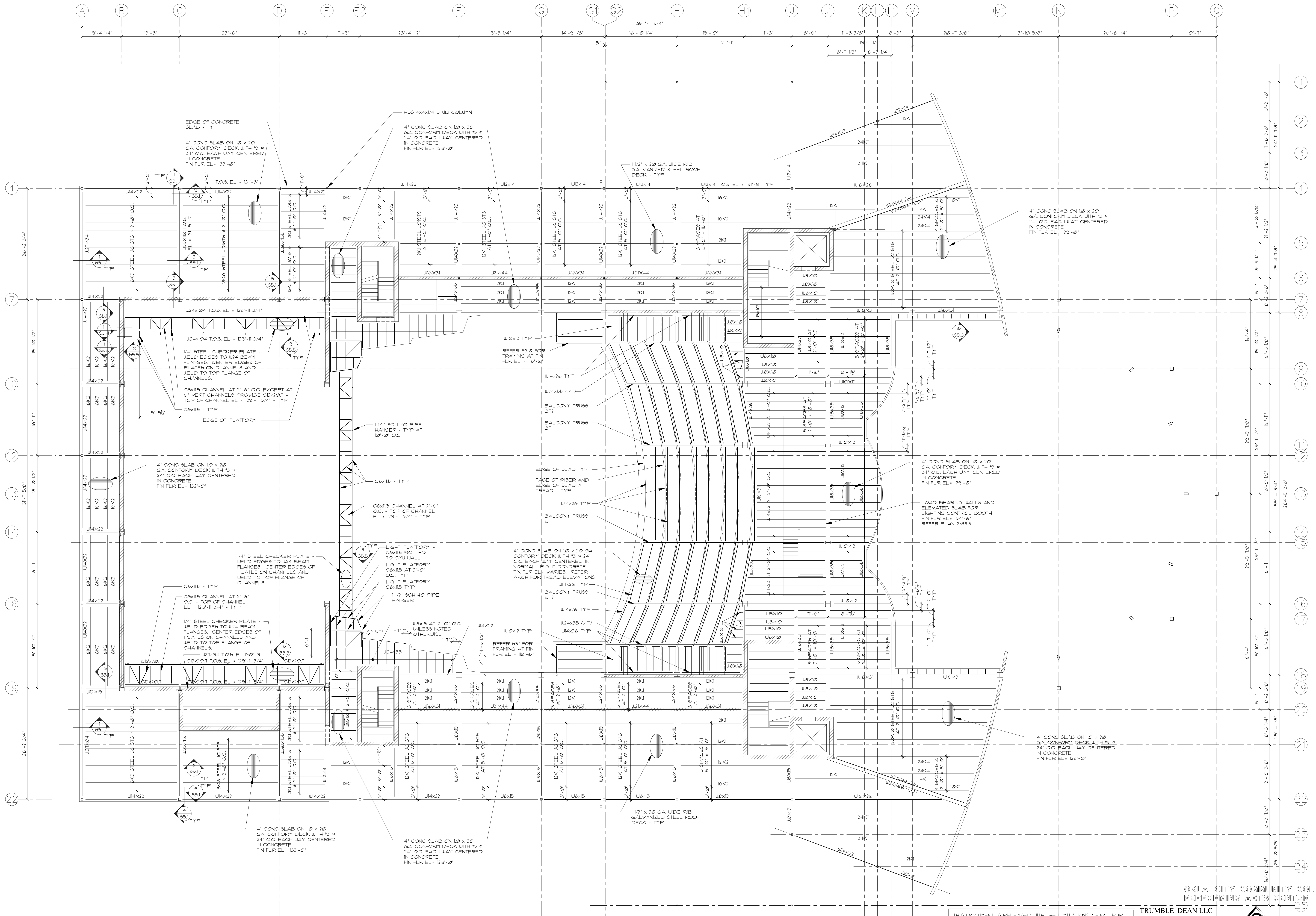
1 BALCONY FLOOR FRAMING PLAN - EL = 129'-0" & 134'-0" SCALE: 1/8" = 1'-0" PLAN NORTH TRUE NORTH
