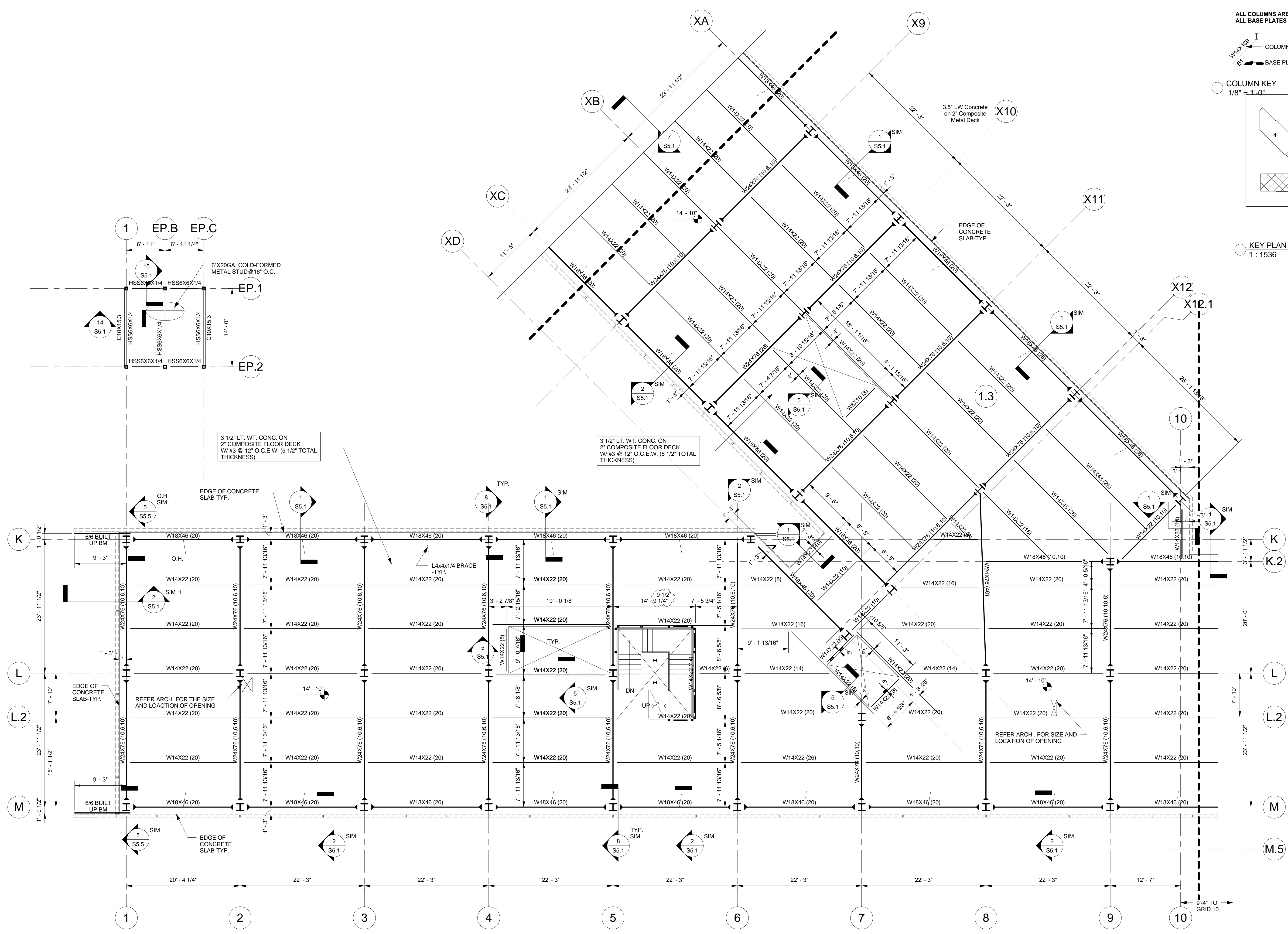
1 2nd Floor Plan Area 3 1/8" = 1'-0"
